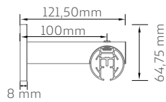
Riel Aeris a pared
